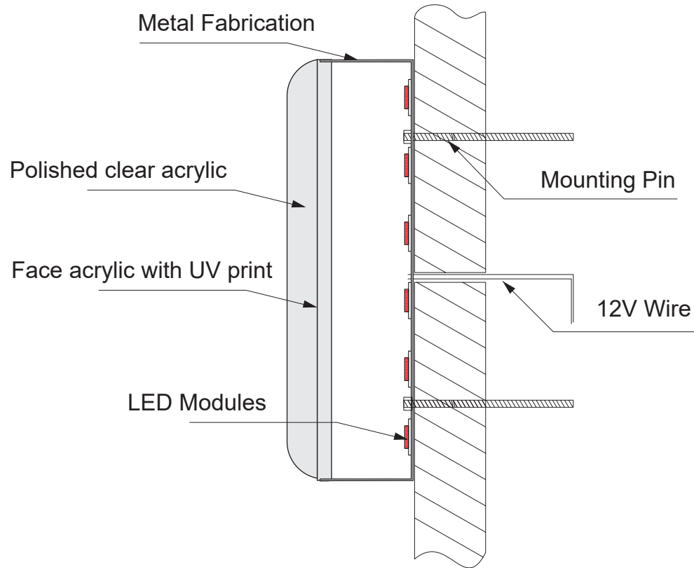
Side View Flush Mount
