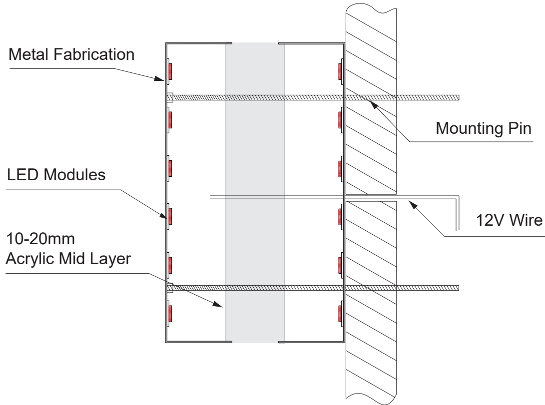
Side View Flush Mount
