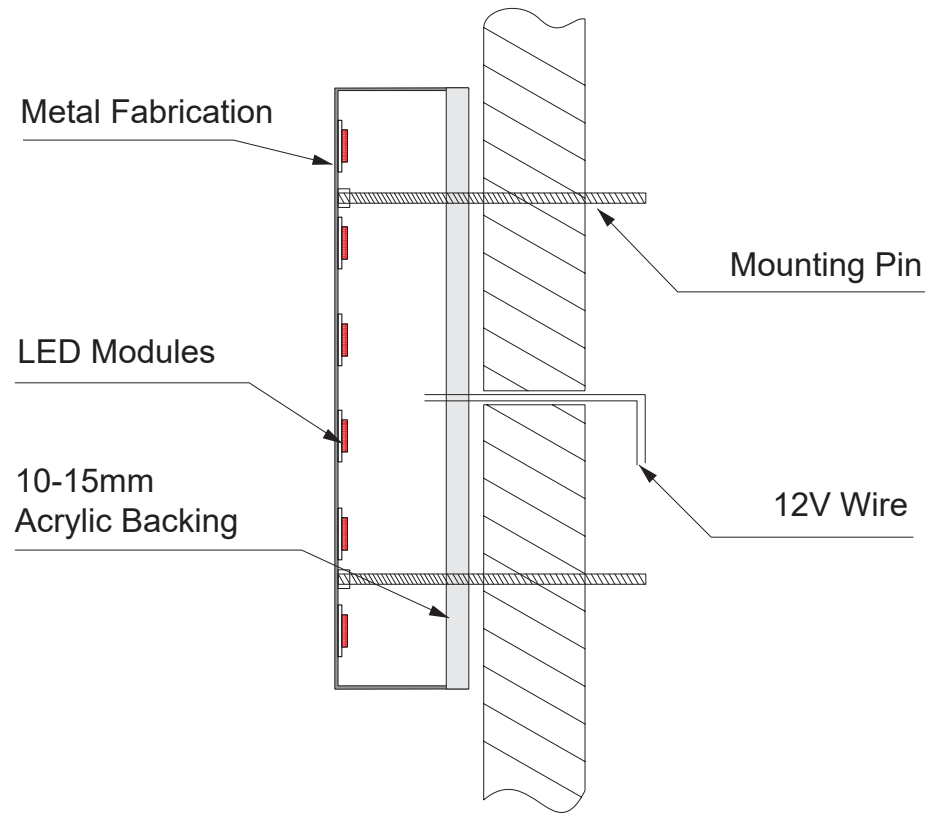
Option B: Stand Off Mounting
