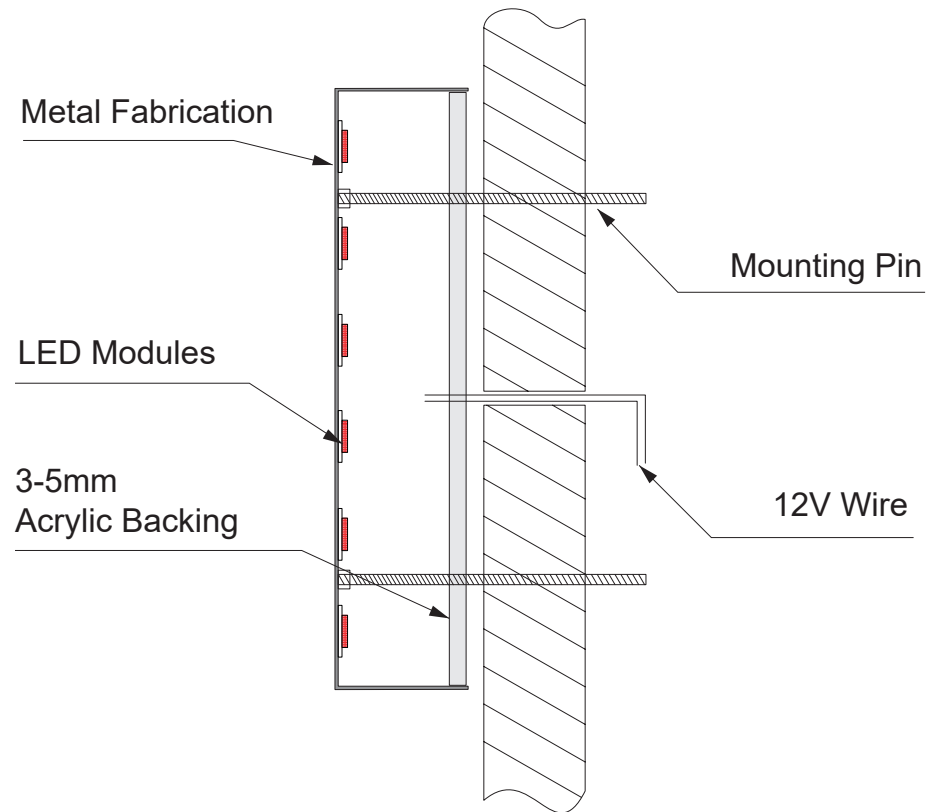
Option B: Close Back
