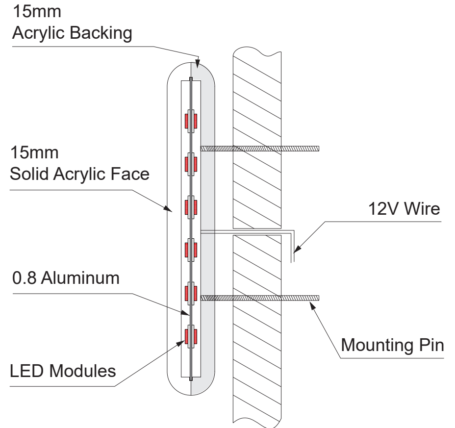
Option D: 360° Neon Sign Stroke \geq 28\text{mm}
