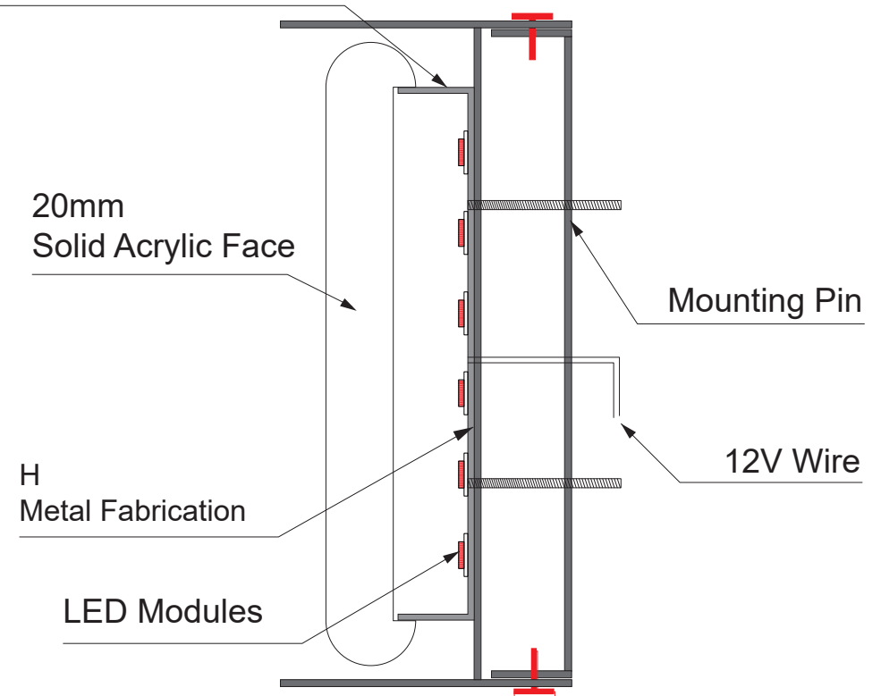
Option H : 270° Neon Sign (H Holder) Closed Backing
