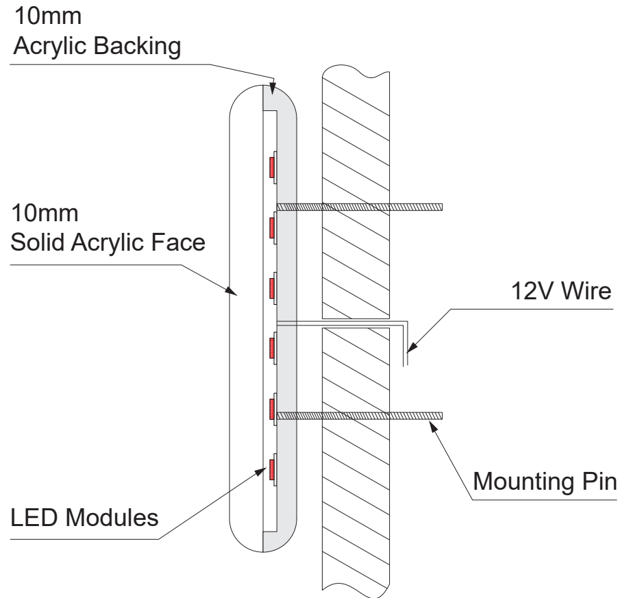
Option C: 360° Neon Sign Stroke \geq 18\text{mm}
