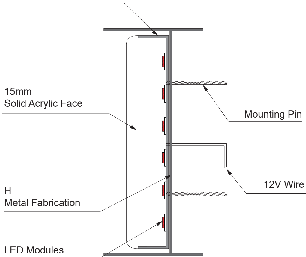
Option E: 180° Neon Sign (H Holder) Open Backing
