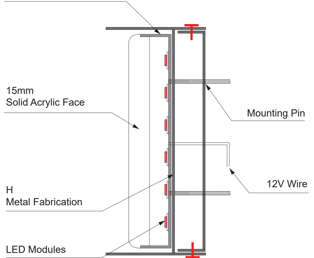
Option F: 180° Neon Sign (H Holder) Closed Backing
